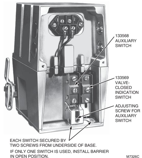
Fig. 2. V4055 Actuator with cover removed.
