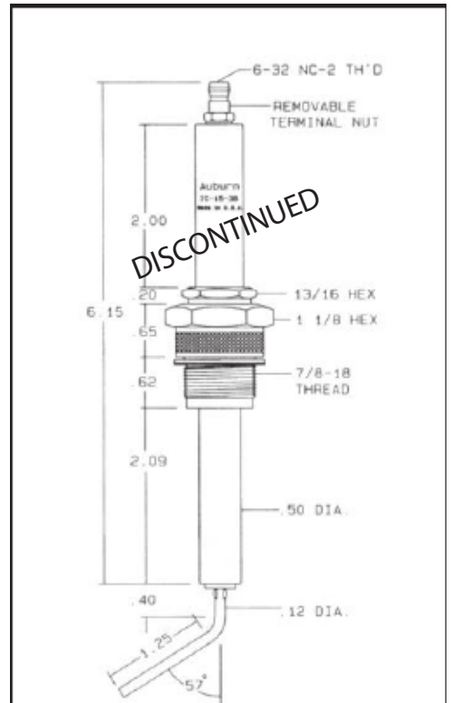
CHROMEL "D" Center Wire
