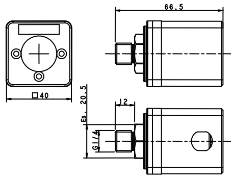
Fig. 3 G1/4 threaded male fixing system
