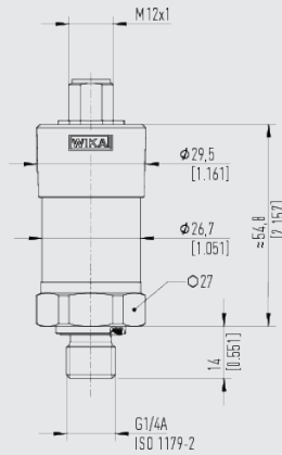
Con conector circular M12 x 1 (4-pin)
